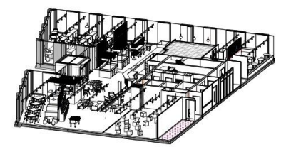
3 3D - Level 00 - View 2
