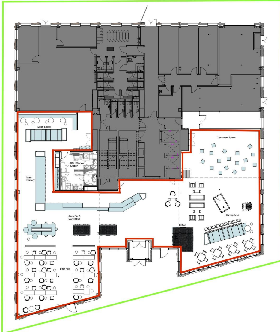
1 Level 00 - General Arrangement 1 : 100
