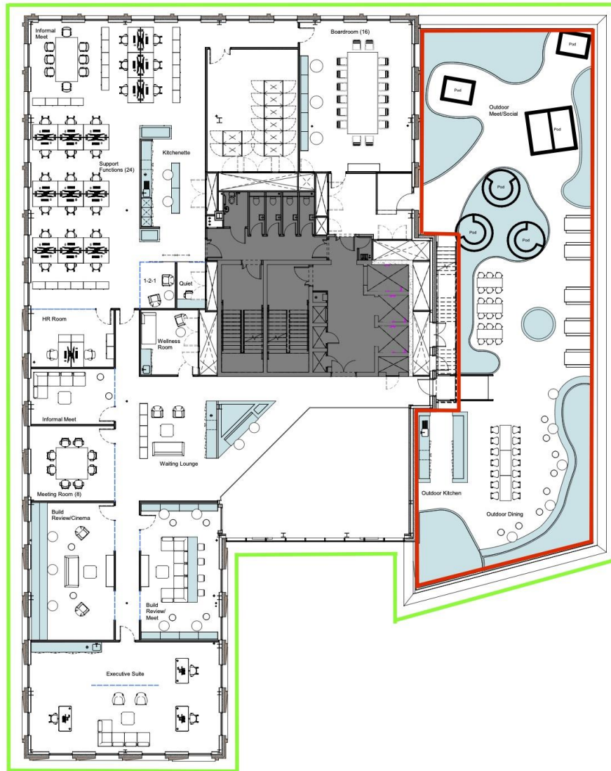
1 Level 05 - General Arrangement 1 : 100
