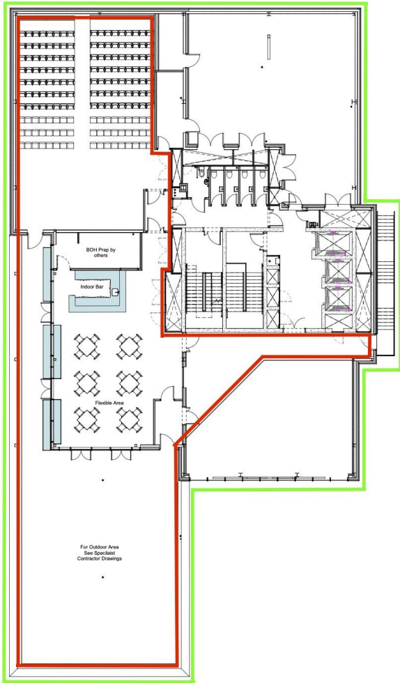
1 Level 06 - General Arrangement 1:100
