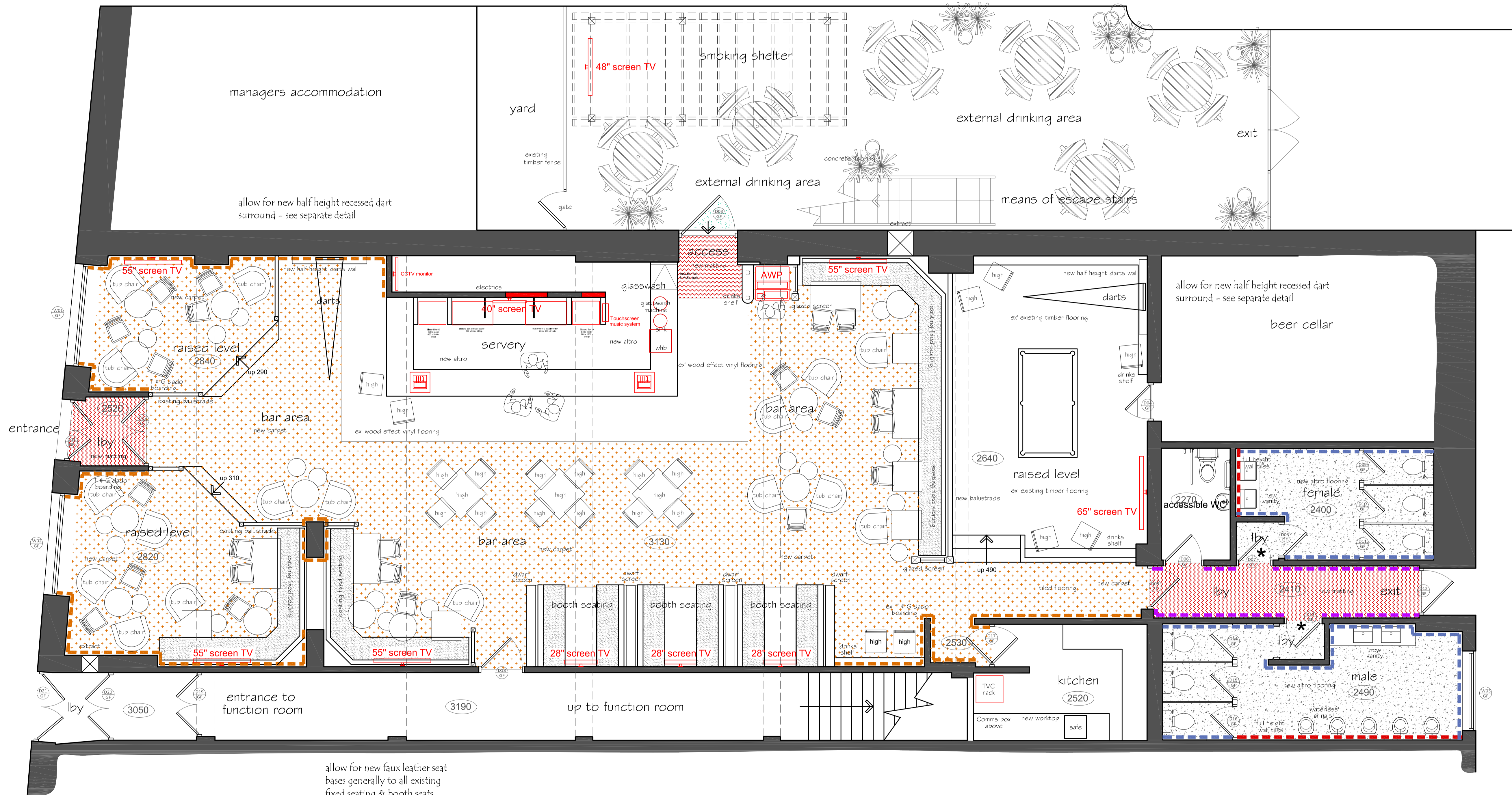
scheme proposals - ground floor layout e.d.a. 182 sqm
